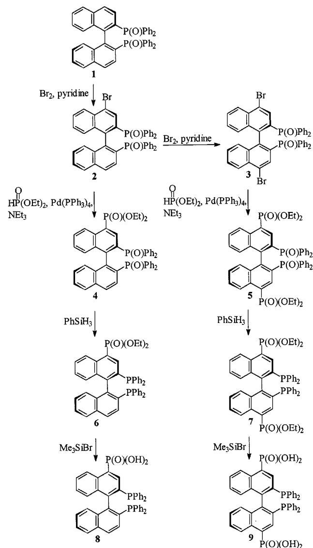
Scheme 1. Synthesis of phosphorylated 2,2'-bis(diphenylphosphanyl)-1,1'-binaphthyls
