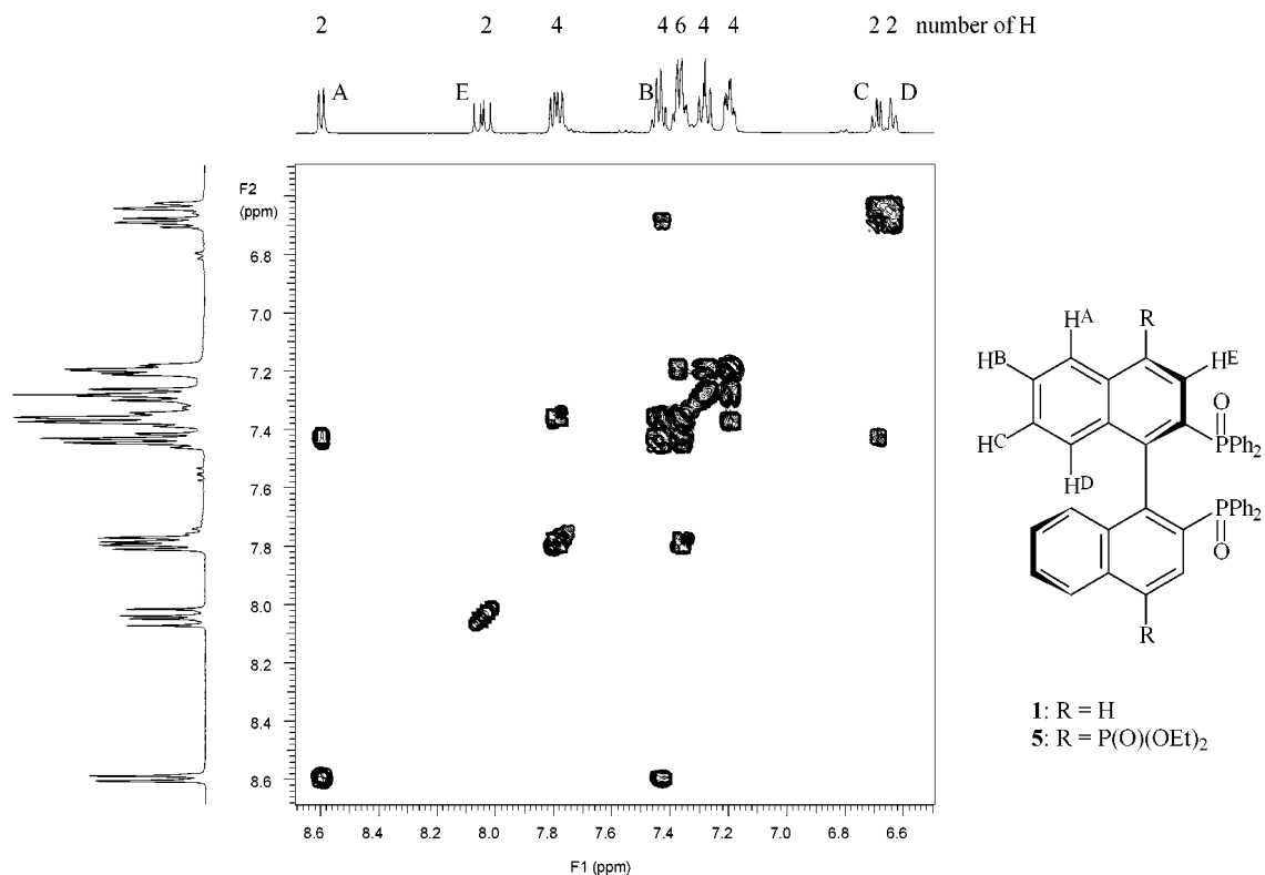
Figure 1. 1 H COSY spectrum of 5
